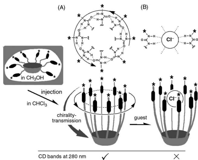
Fig. 2 Schematic representations for the self-folding of 1 . In chloroform, the urea moieties (black ovals) of 1 form intramolecular hydrogen bonds clockwise or counterclockwise in a cyclic fashion, the direction of which is controlled by the neighboring chiral termini. A chirality transmission from the chiral urea termini to the macrocycles through hexyl spacers results in CD bands at 280 nm, in the absorption wavelength range of the macrocyclic skeleton (A). Intermolecular hydrogen bonds with an encapsulated anion ( \text{Cl}^- ), resulting in the decrease and disappearance of the CD bands at 280 nm (B). Each asterisk (*) represents a chiral center.
