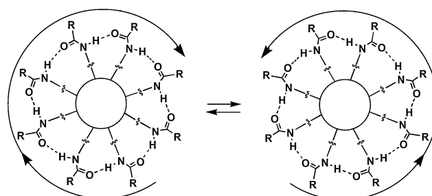
Fig. 1 Head-to-tail hydrogen-bonded belt formed cooperatively by eight amide groups of Rebek's self-folding cavitant. Interconversion of two cycloenantiomers, with clockwise and counterclockwise orientation of the amide bonds, is shown. The large circles represent the resorcinarene skeleton; R is an alkyl group.
