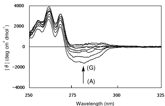
Fig. 8 CD spectra of 1-S in chloroform in the presence of \text{Cl}^- (as a tetrabutylammonium salt): 0, 2, 7, 12, 22, 31, and 36 equiv. (from A to G).
