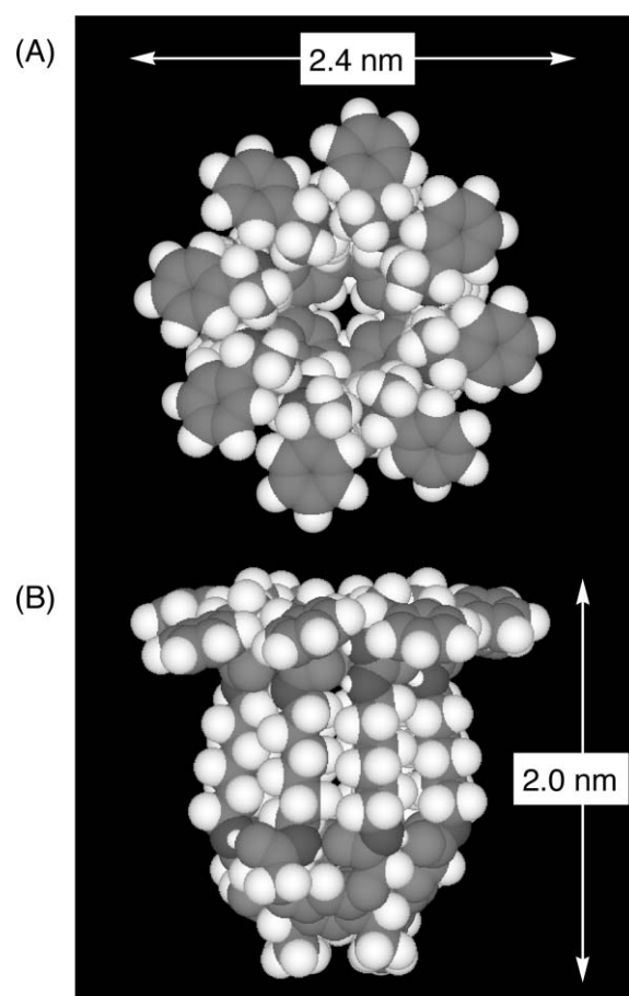
Fig. 3 A space-filling representation of 1-R . Top view (A) and side view (B). The undecyl groups are replaced by methyl groups for clarity.
