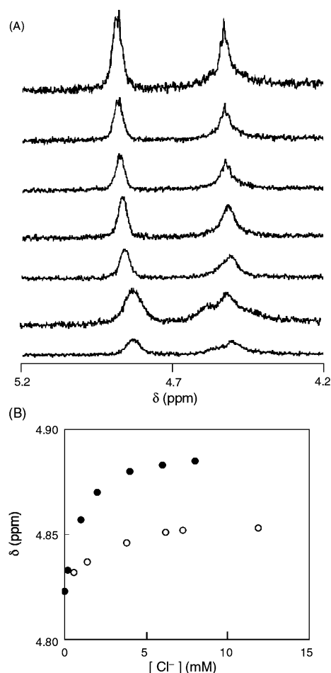
Fig. 7 Partial ^1\text{H} NMR spectra of 1-S at 298 K in the presence of \text{Cl}^- (as a tetrabutylammonium salt): 0, 1, 5, 10, 20, 30, and 40 equiv. (from bottom to top) (A). The corresponding NMR titration curves for \text{Cl}^- (●) and \text{Br}^- (○) (B).
