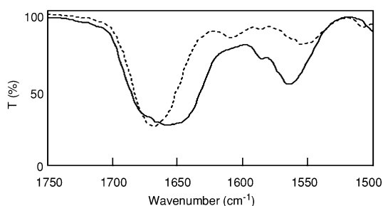
Fig. 4 FT-IR spectra of 1-S (solid line) and 10-S (dotted line) in chloroform at 298 K.
