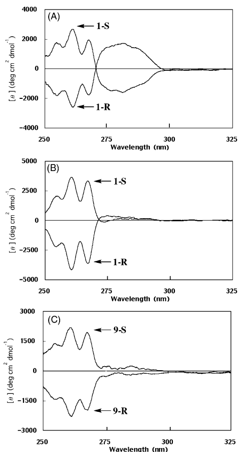
Fig. 6 CD spectra of 1-S and 1-R in chloroform (A) or in chloroform–methanol (3 : 97 v/v) (B). CD spectra of 9-S and 9-R in chloroform (C).
