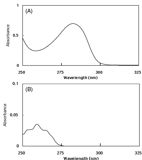
Fig. 5 UV spectra of 1-S (A) and 11-S (B) in chloroform.
