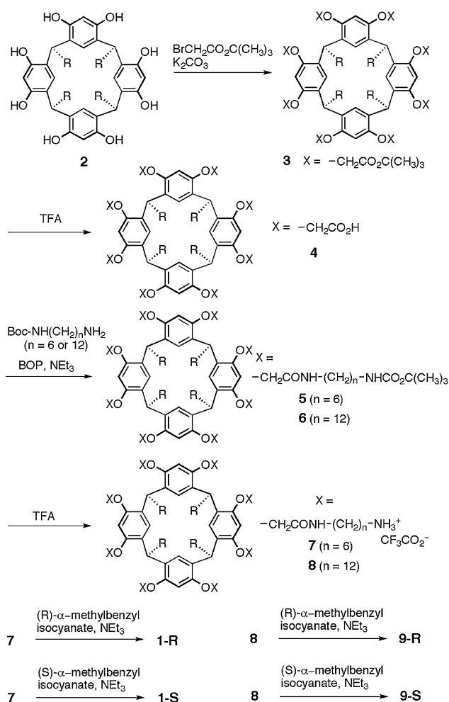
Scheme 1 Preparation of urea-functionalized resorcinarenes ( R = (\text{CH}_2)_{10}\text{CH}_3 ).
